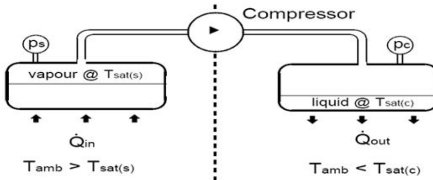
p_c = Condenser or ‘high side’ pressure. p_s = Evaporator, ‘low side’, or suction pressure. Figure 6: Heat pumps.
