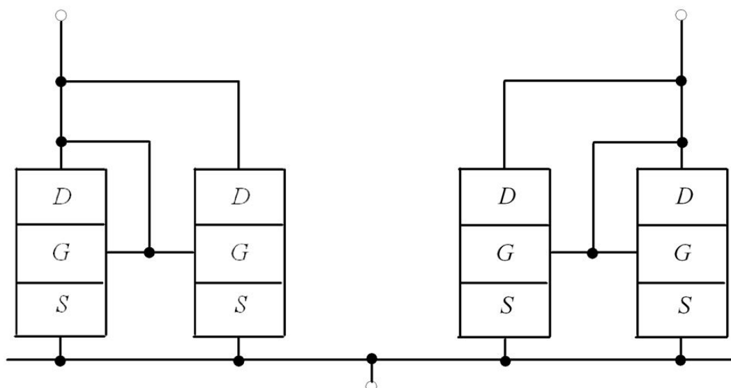
Figure 1: The considered current comparator [4]
