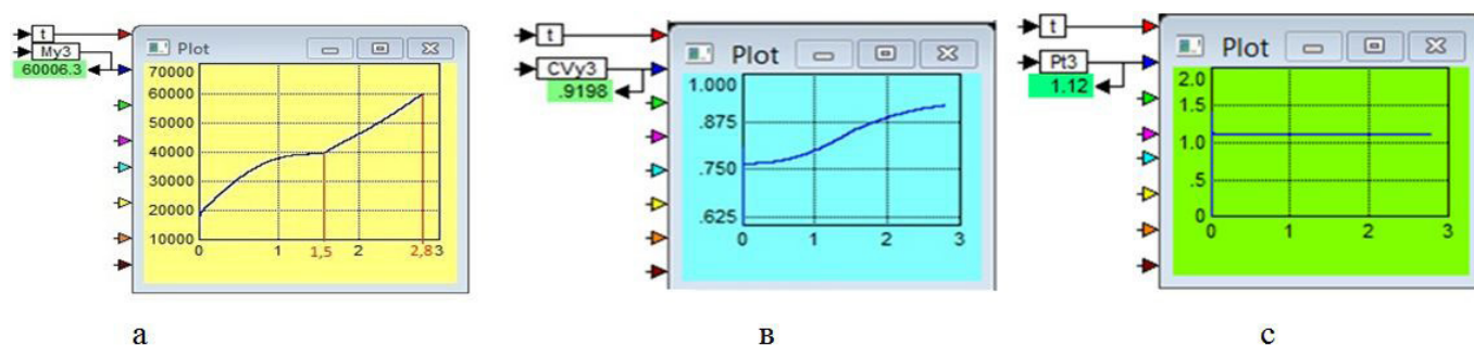
Figure 1: Graphic interpretation of the offered method (a - mass massecuite (Mu3); b - concentration massecuite (CVu3); c - coefficient of supersaturation (Pt3).
