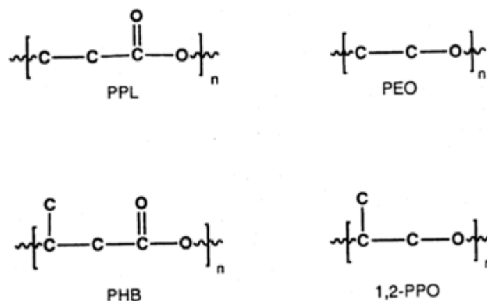
Figure 7: Backbone structures of salt-solvating polymers. The figure shows the similarity of backbone structure, with optimal spacing between electron-donating oxygens, of polymers that form ion-conducting salt complexes.
