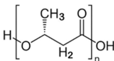
Figure 4: Chemical structure of R-3-polyhydroxybutyrates (PHB). Hydrophobic methyl groups alternate with hydrophilic ester groups.
